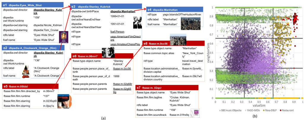
Fig. 1. (a) Movies, directors, and locations from DBpedia (blue) and Freebase (red), where e_1, e_2, e_3 , and e_4 match with e_7, e_5, e_6 , and e_8 , respectively. (b) Value and neighbor similarity distribution of matches in four datasets.
